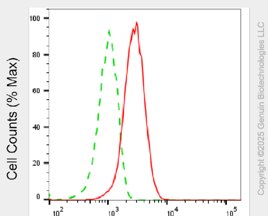
Creatine kinase B-Alexa Fluor® 647
